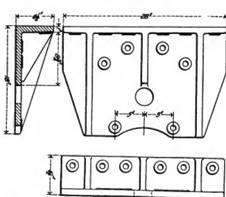
Figs. 3679-3681. Front End Sill Bottom Corner Casting.
